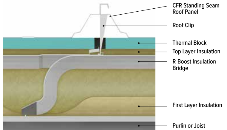
R-Boost Roof Assembly
